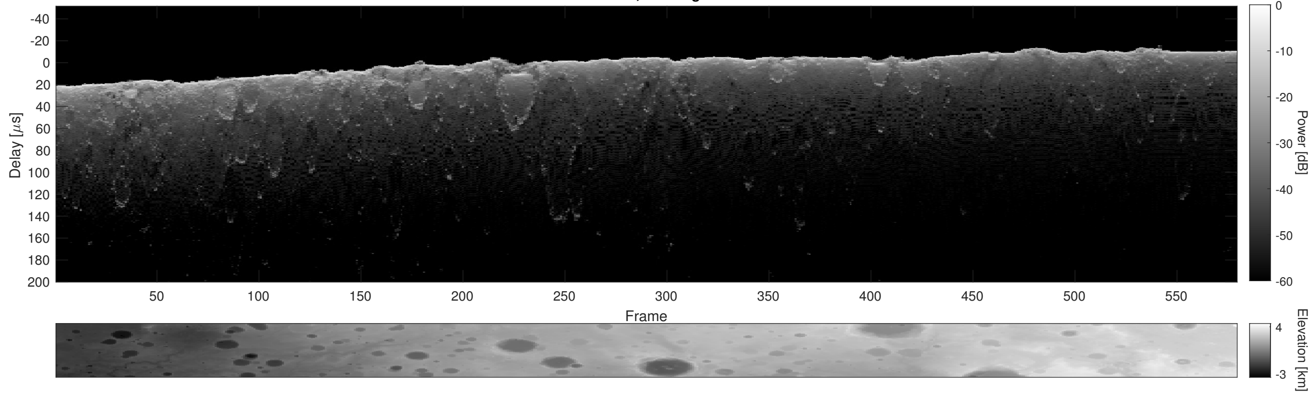
Orbit 4722, Cluttergram
