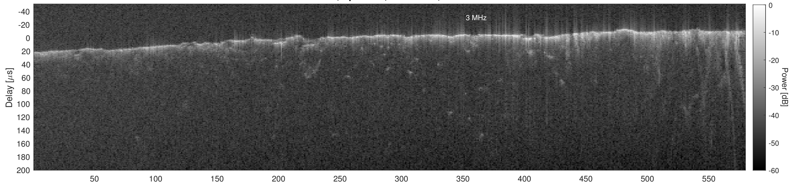
Orbit 4722, Cluttergram
