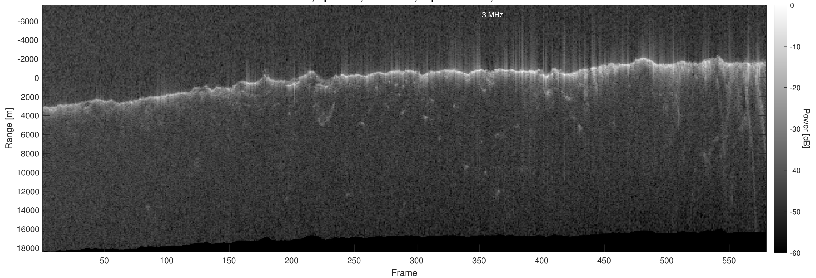
Orbit 4722, Optimized, No Window, Depth-Corrected, Channel 2
