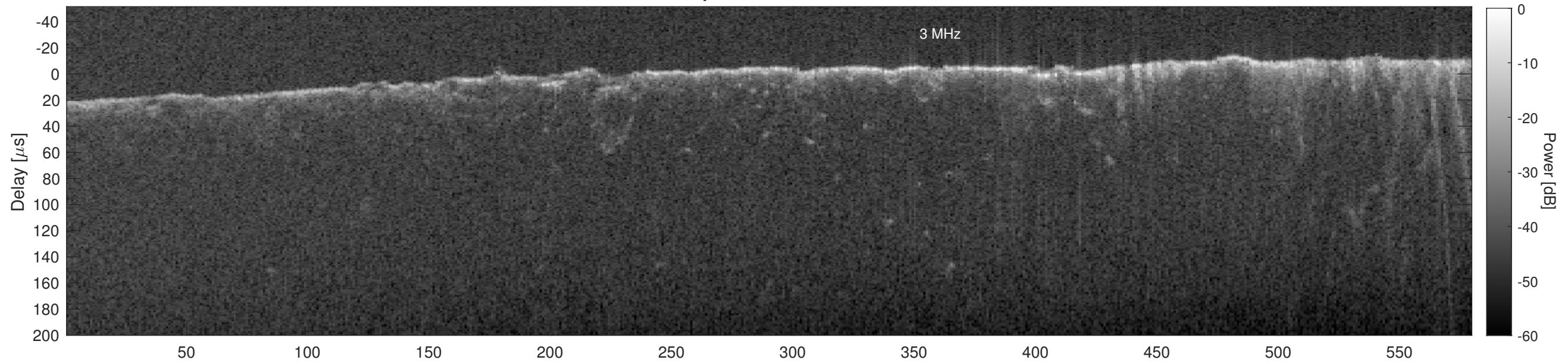
Orbit 4722, Cluttergram
