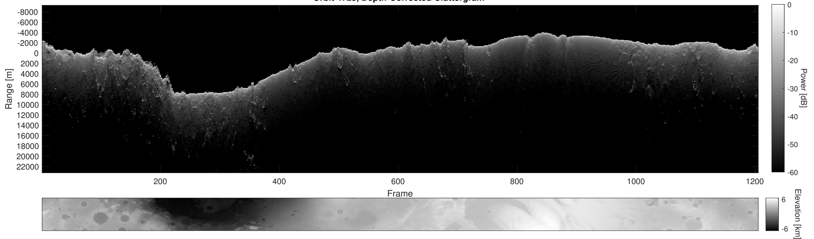
Orbit 4725, Depth-Corrected Cluttergram
