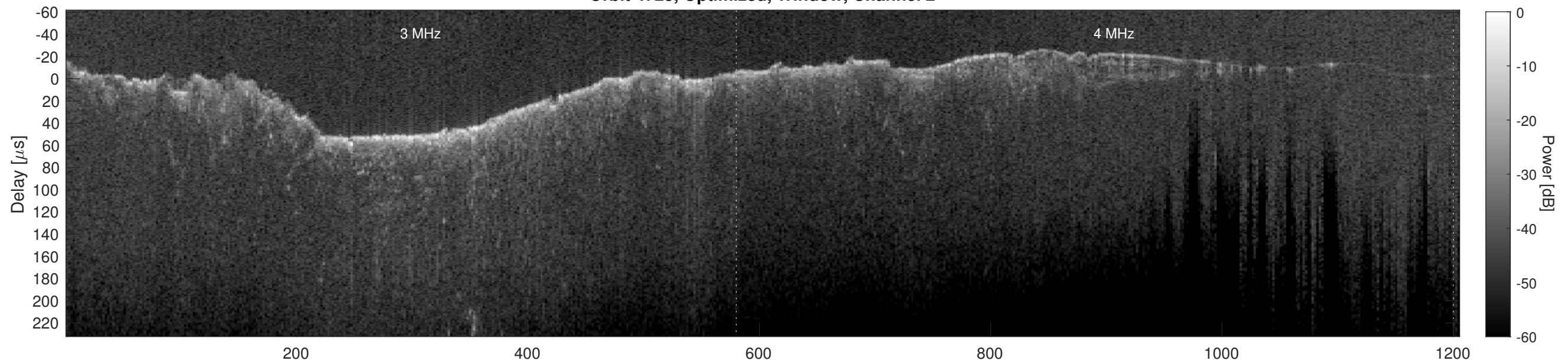
Orbit 4725, Cluttergram
