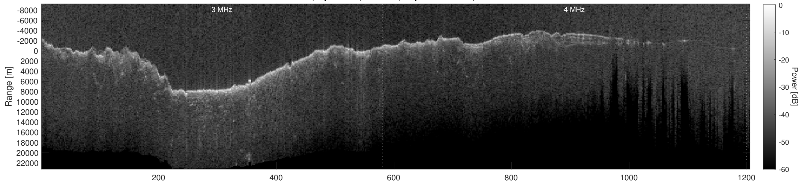
Orbit 4725, Depth-Corrected Cluttergram
