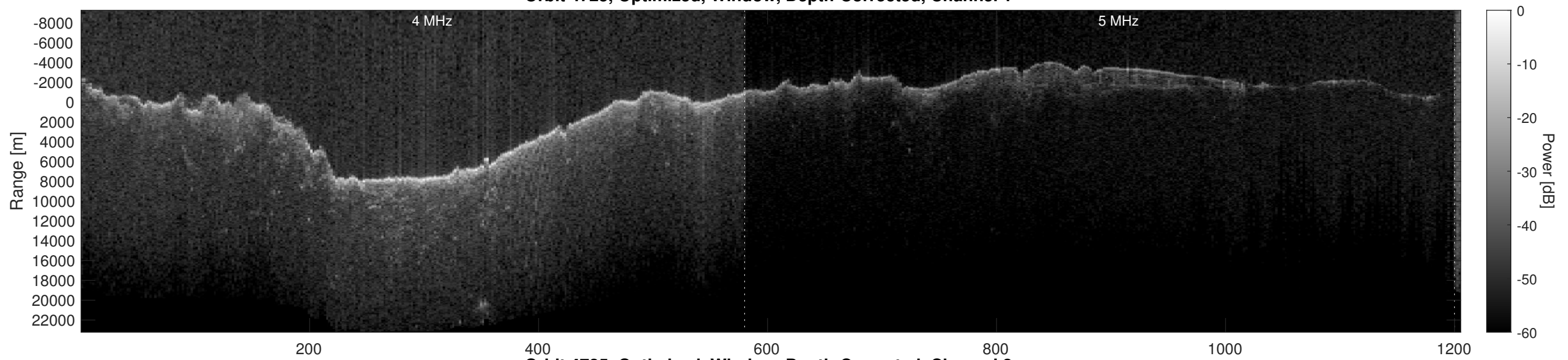
Orbit 4725, Optimized, Window, Depth-Corrected, Channel 2
