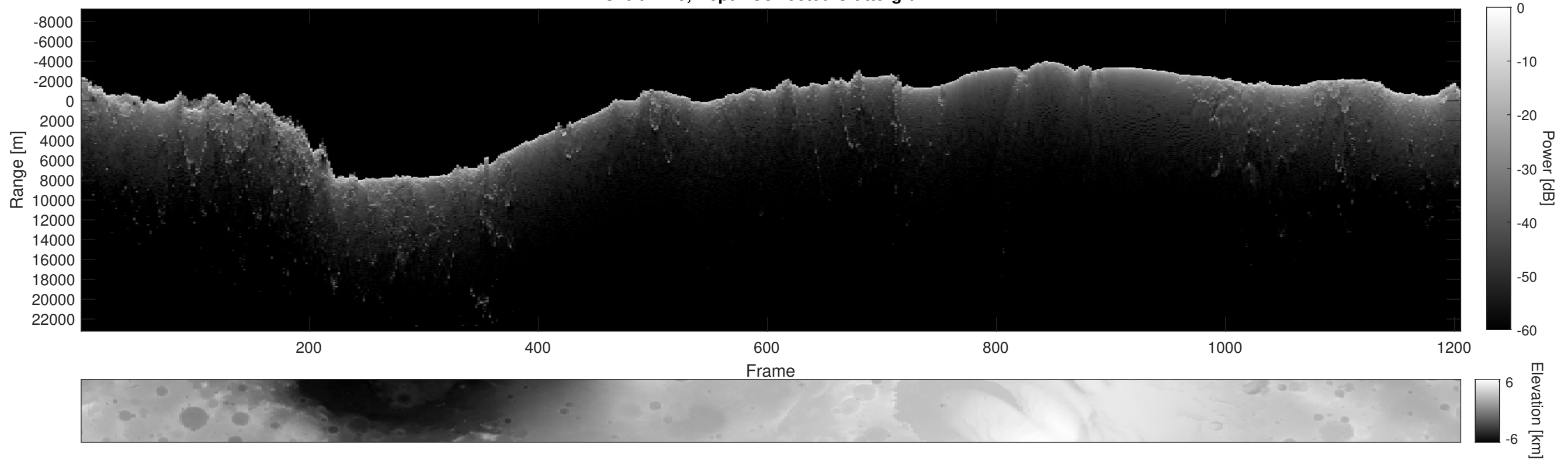
Orbit 4725, Depth-Corrected Cluttergram
