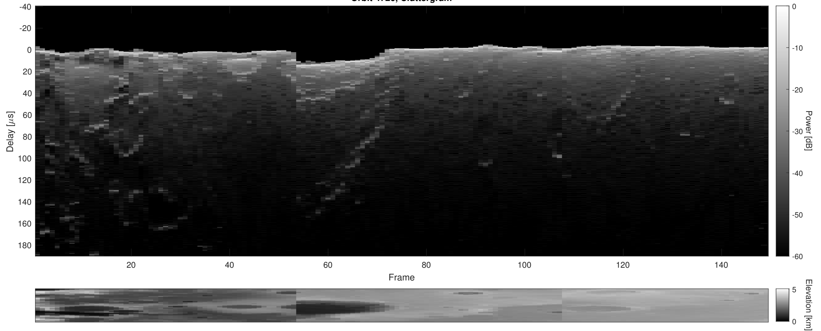
Orbit 4726, Cluttergram
