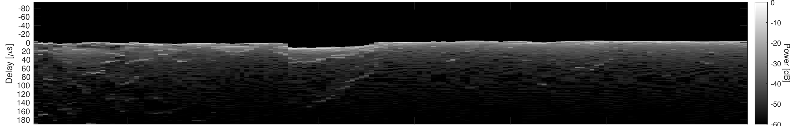
Orbit 4726, Cluttergram
