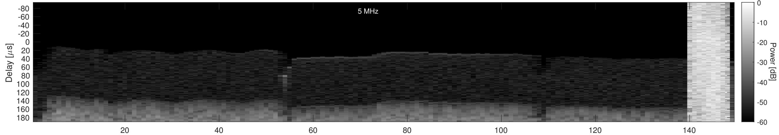
Orbit 4726, Cluttergram
