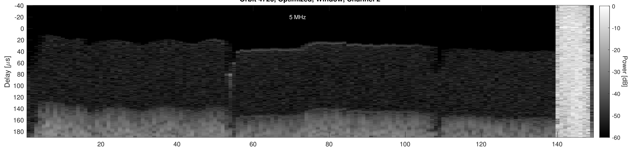
Orbit 4726, Cluttergram
