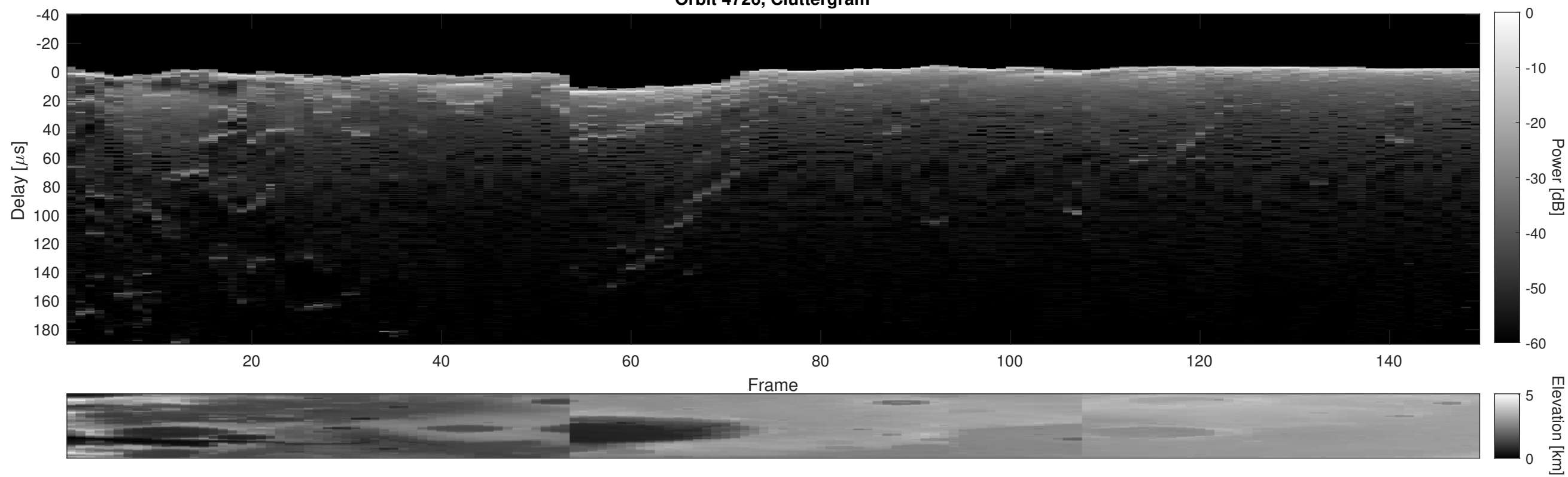
Orbit 4726, Cluttergram
