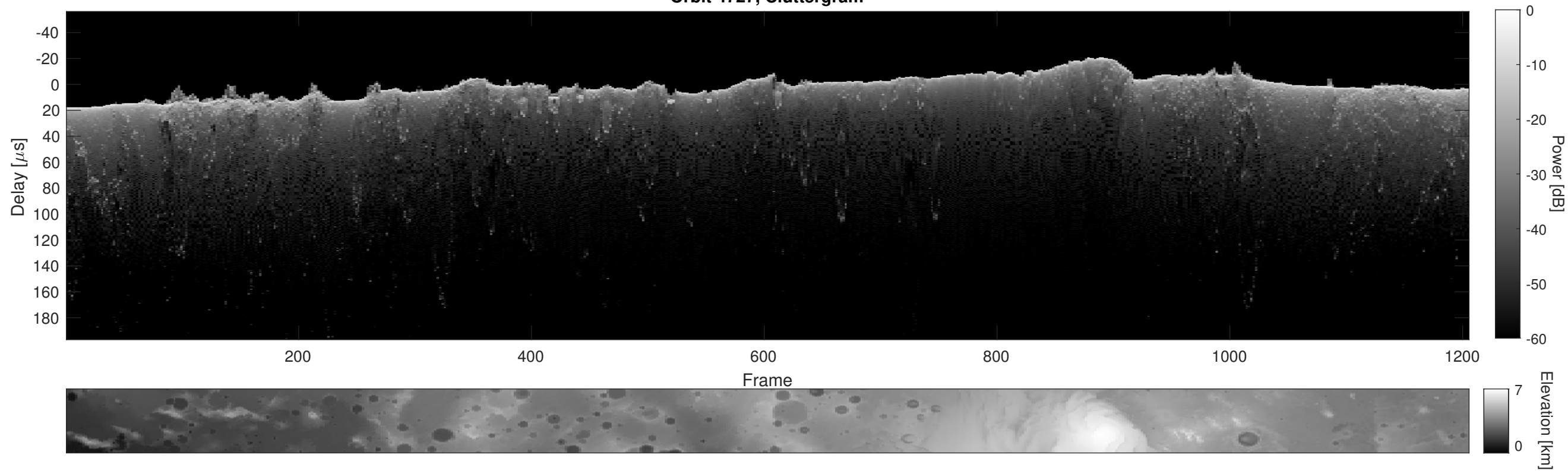
Orbit 4727, Cluttergram
