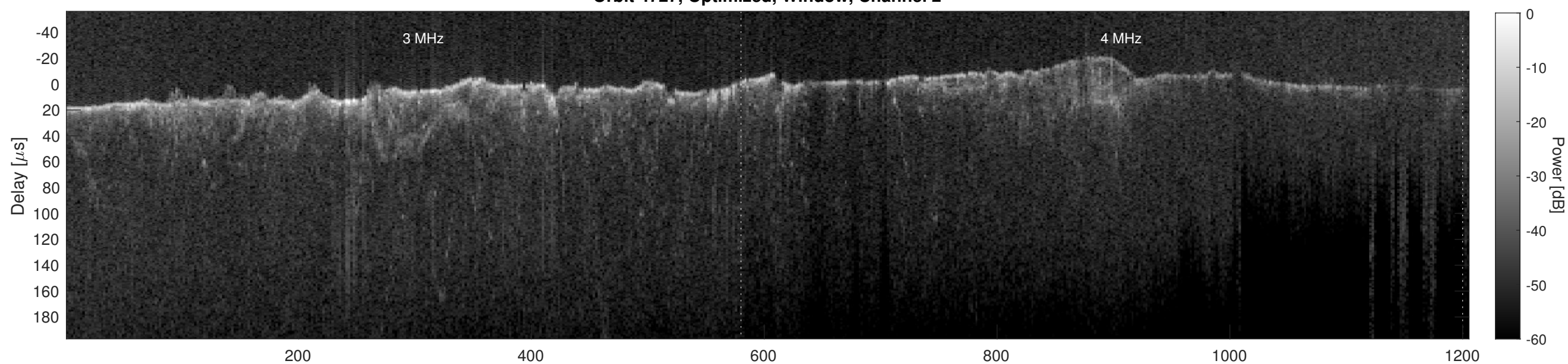
Orbit 4727, Cluttergram
