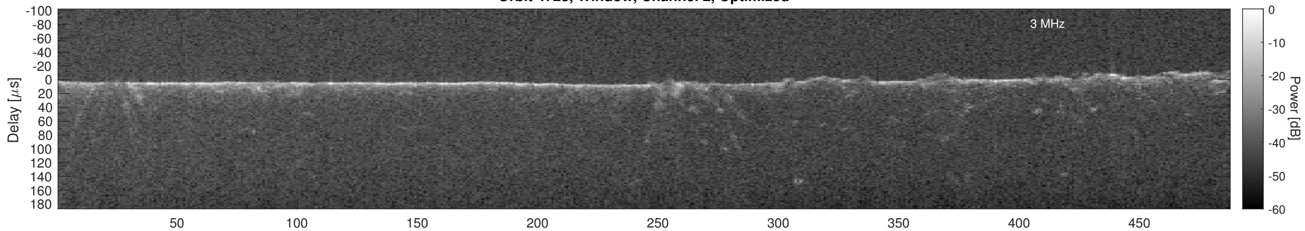
Orbit 4728, Cluttergram
