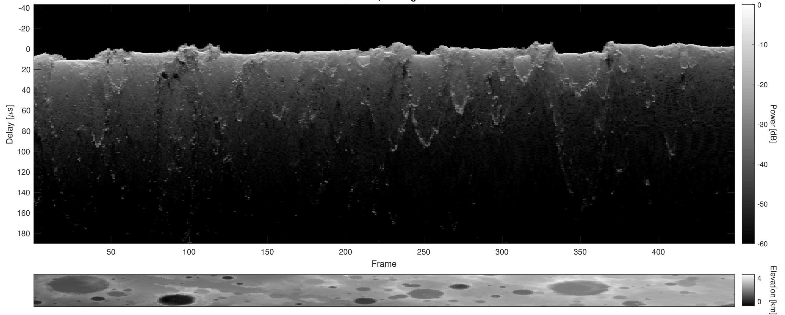
Orbit 4729, Cluttergram
