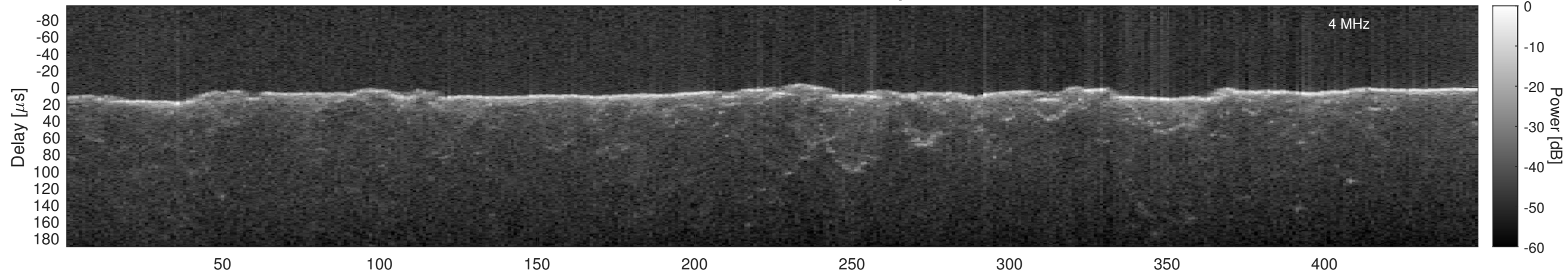
Orbit 4729, Window, Channel 1, Optimized
