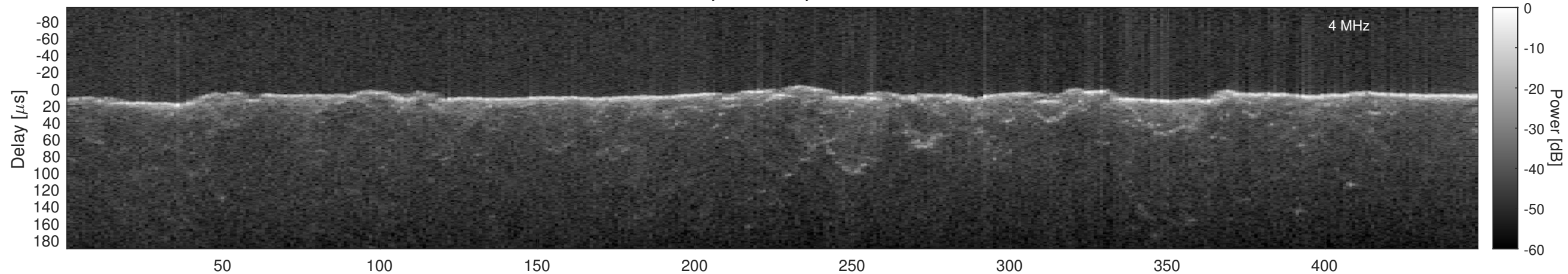
Orbit 4729, Window, Channel 1, Chapman
