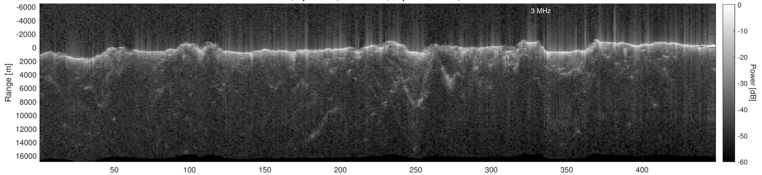
Orbit 4729, Depth-Corrected Cluttergram
