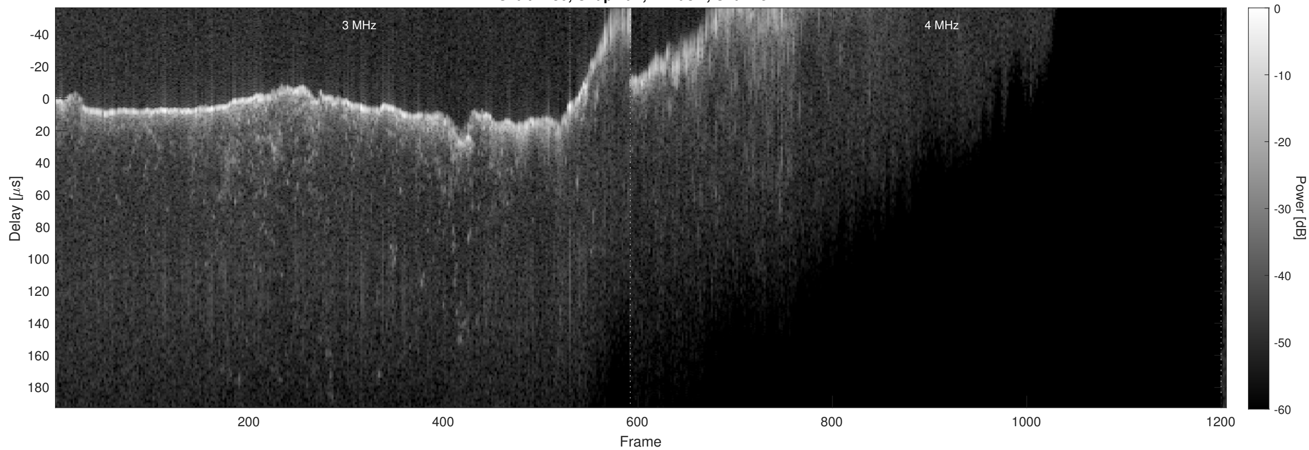
Orbit 4730, Chapman, Window, Channel 2
