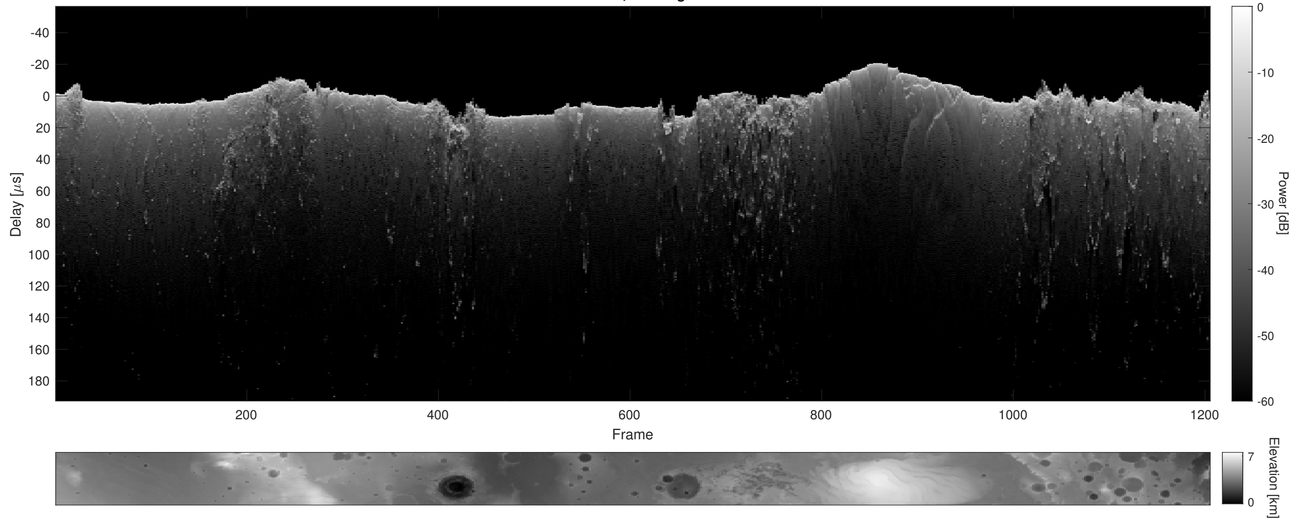
Orbit 4730, Cluttergram
