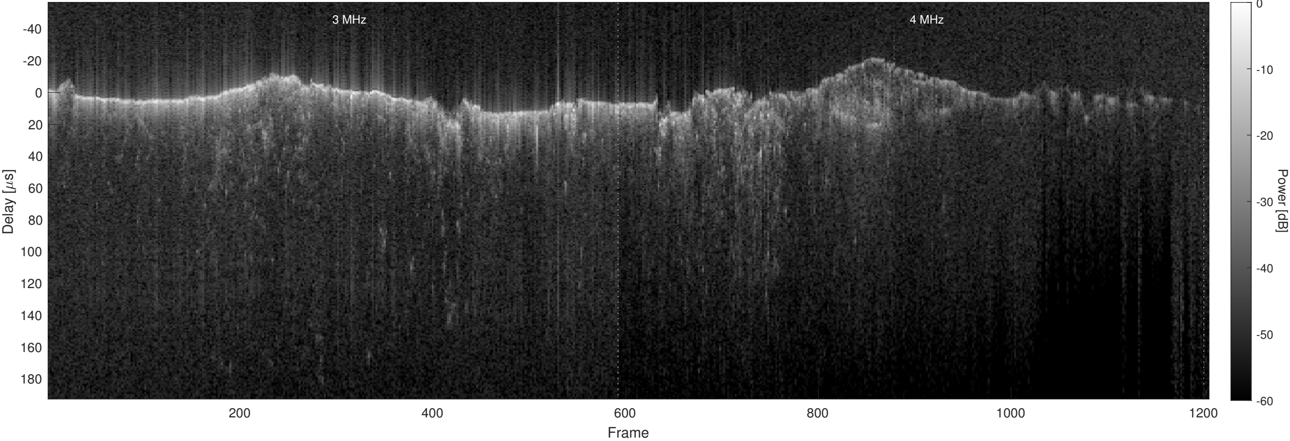
Orbit 4730, Optimized, No Window, Channel 2
