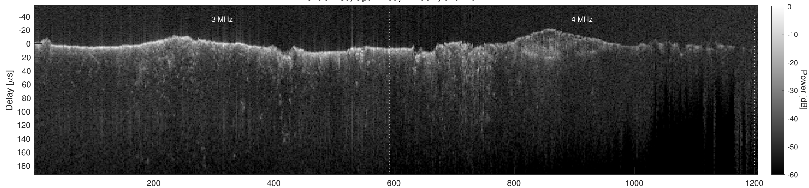
Orbit 4730, Cluttergram
