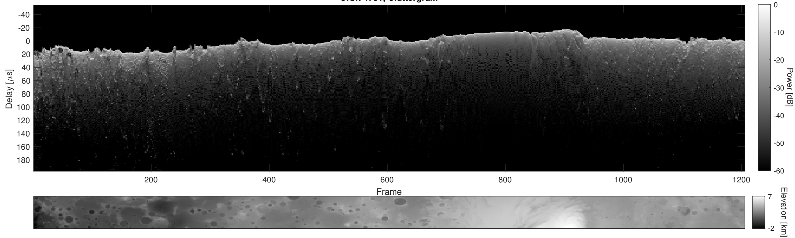
Orbit 4731, Cluttergram
