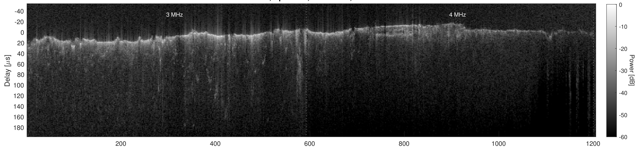
Orbit 4731, Cluttergram
