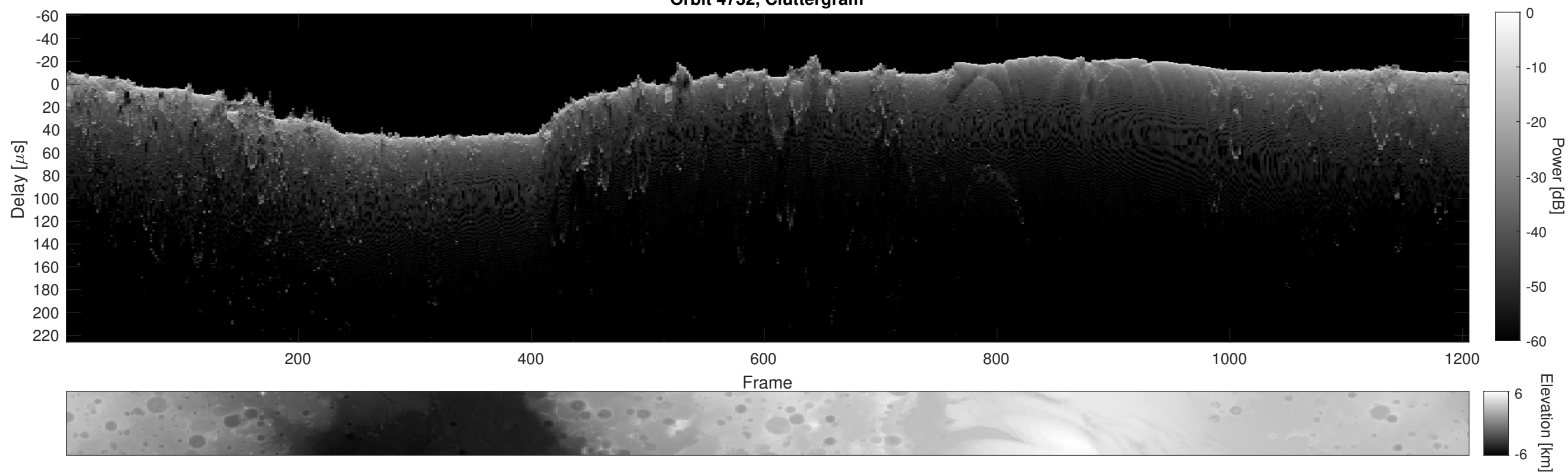
Orbit 4732, Cluttergram
