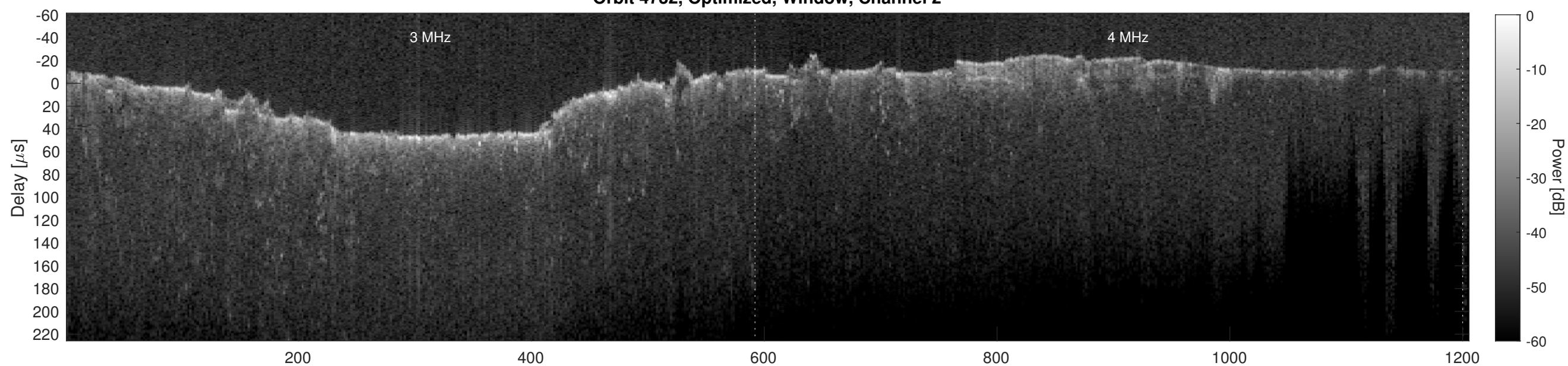
Orbit 4732, Cluttergram
