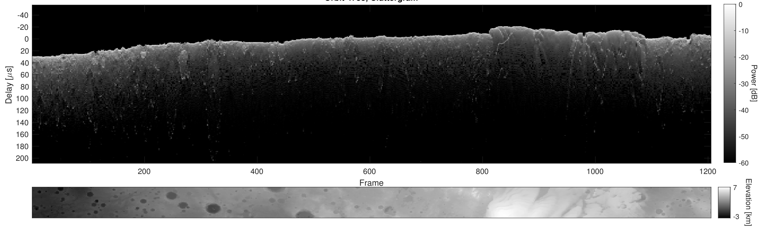
Orbit 4733, Cluttergram
