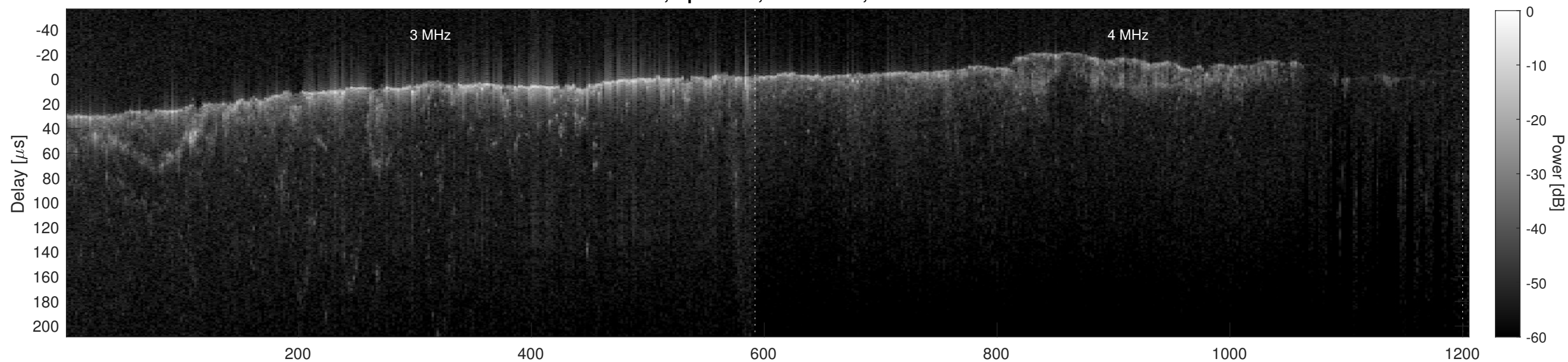
Orbit 4733, Cluttergram
