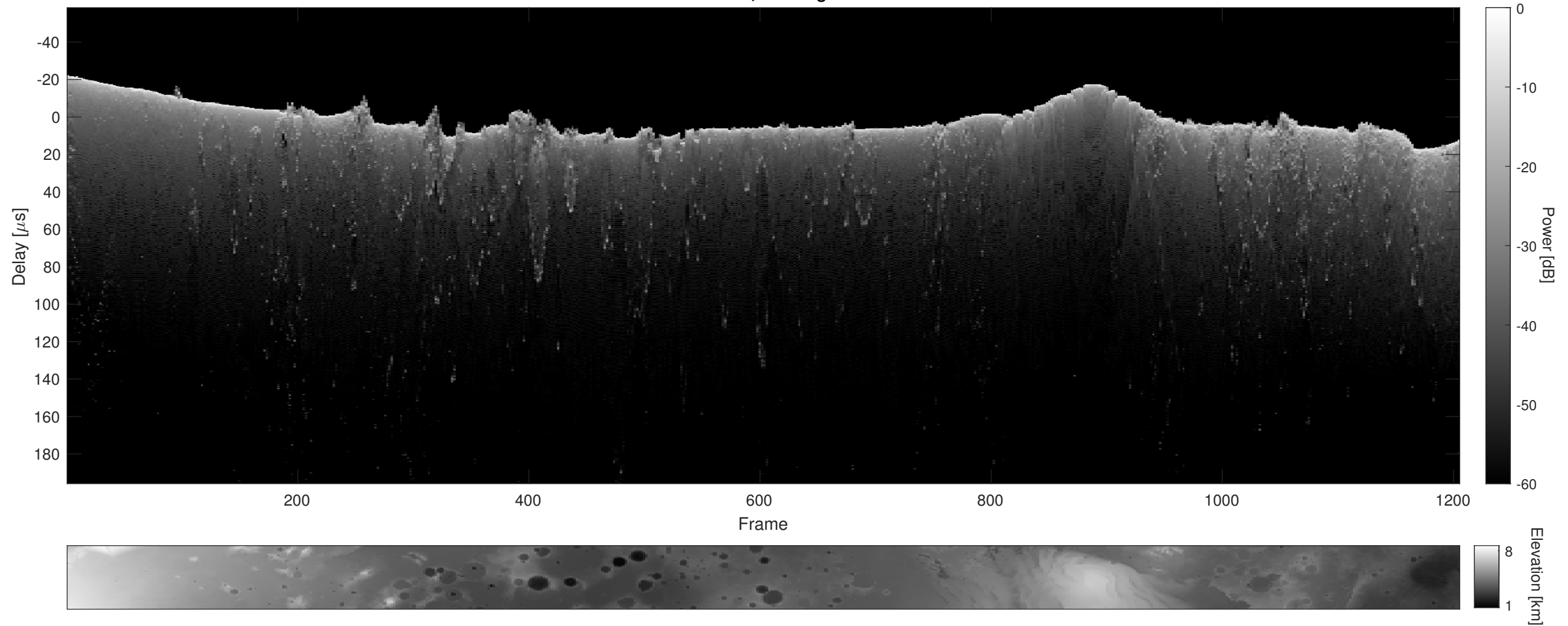
Orbit 4734, Cluttergram
