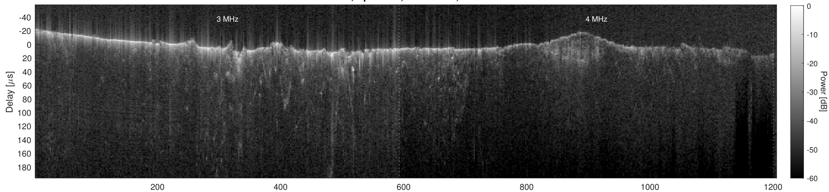
Orbit 4734, Cluttergram
