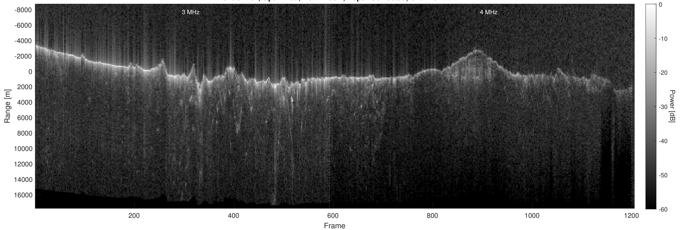
Orbit 4734, Optimized, No Window, Depth-Corrected, Channel 2
