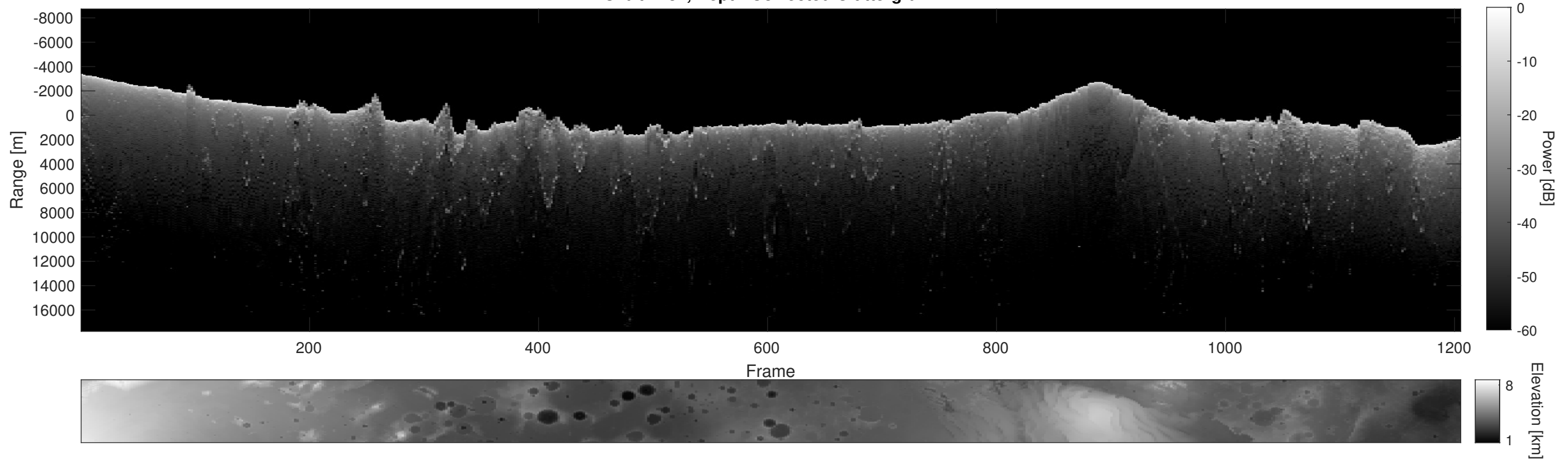
Orbit 4734, Depth-Corrected Cluttergram
