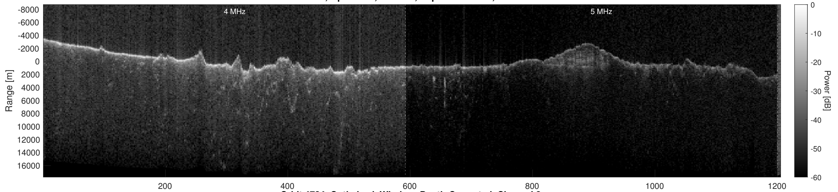
Orbit 4734, Optimized, Window, Depth-Corrected, Channel 2
