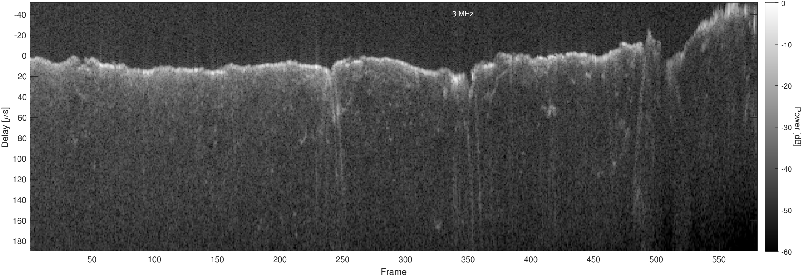
Orbit 4735, Chapman, Window, Channel 2
