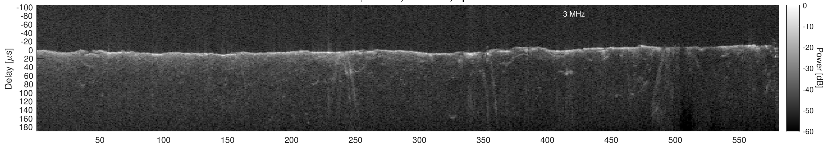
Orbit 4735, Cluttergram
