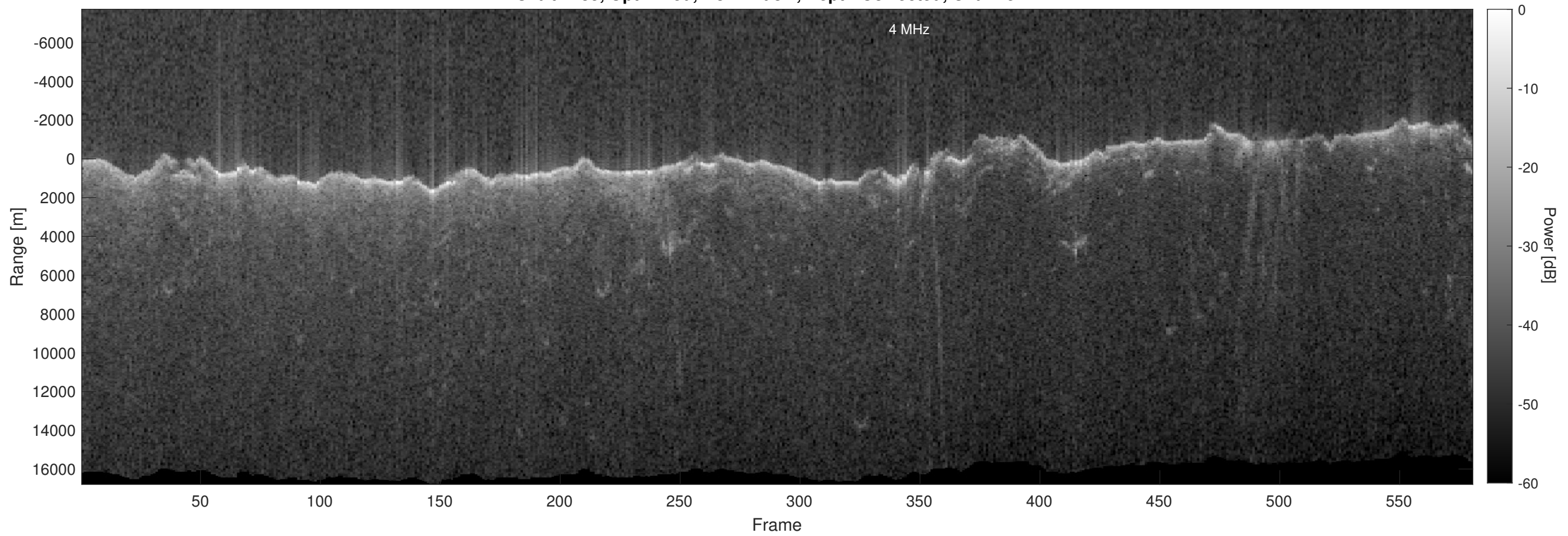
Orbit 4735, Optimized, No Window, Depth-Corrected, Channel 2
