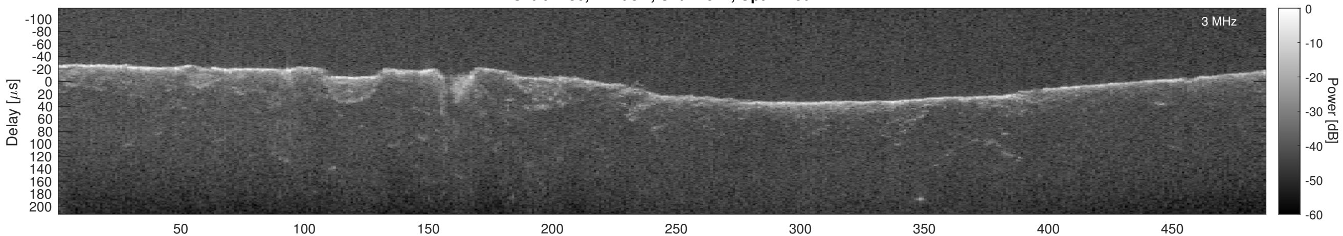
Orbit 4736, Cluttergram
