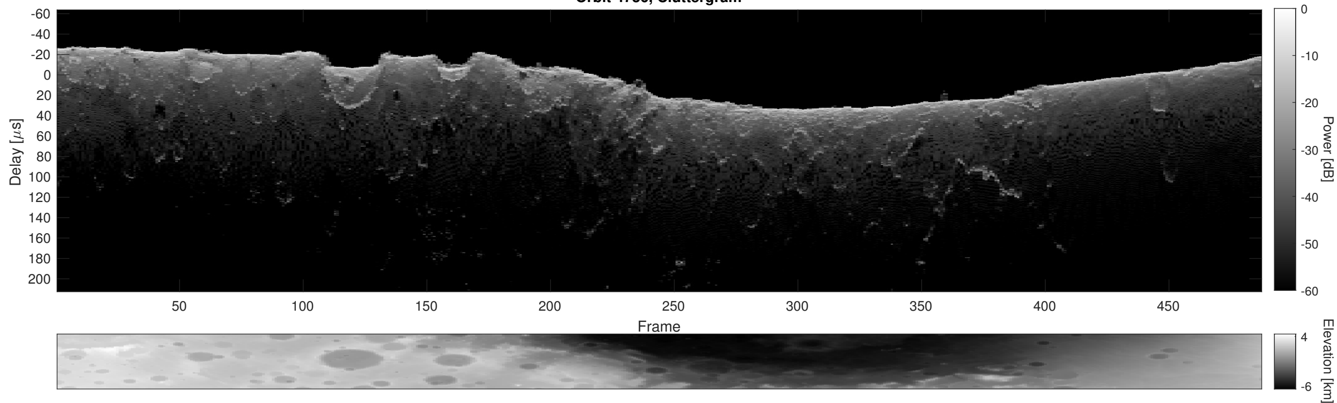
Orbit 4736, Cluttergram
