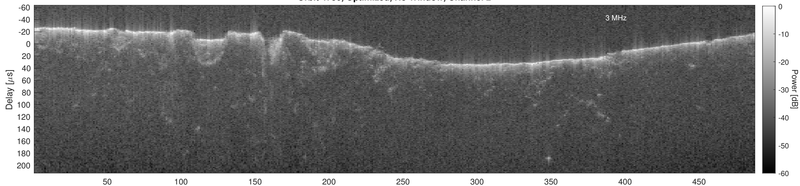
Orbit 4736, Cluttergram
