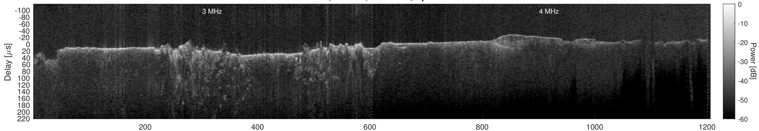
Orbit 4737, Cluttergram
