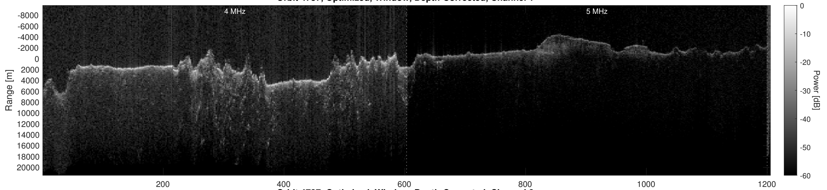
Orbit 4737, Optimized, Window, Depth-Corrected, Channel 2
