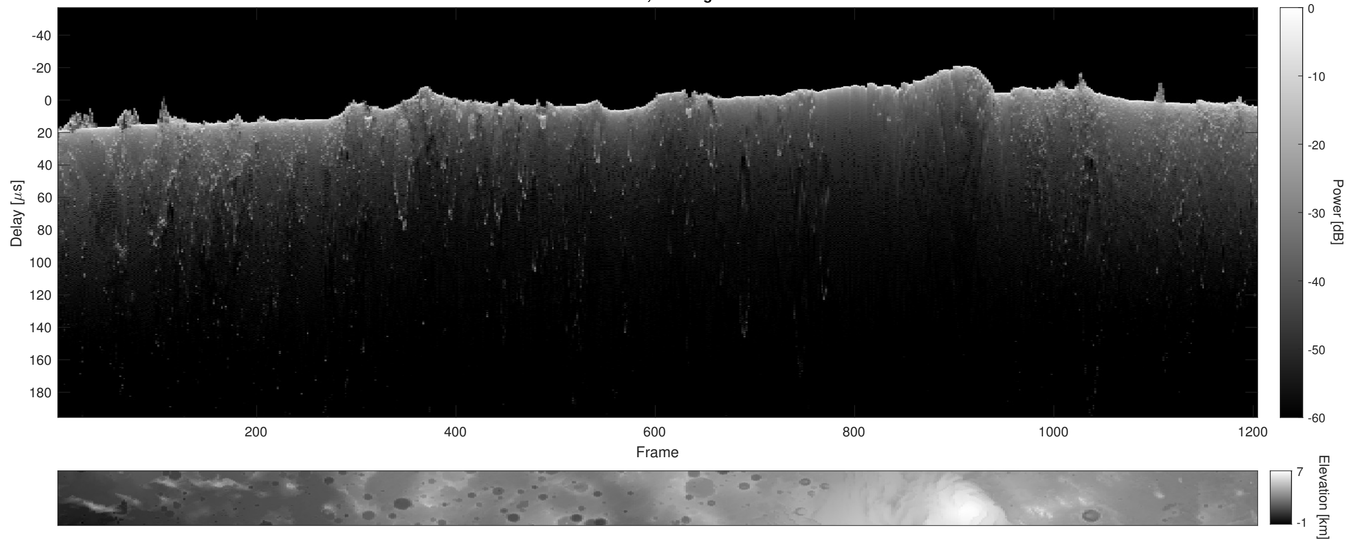
Orbit 4738, Cluttergram
