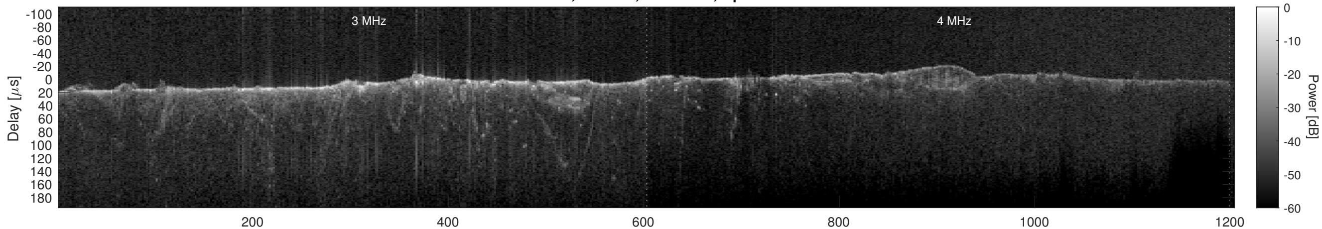
Orbit 4738, Cluttergram
