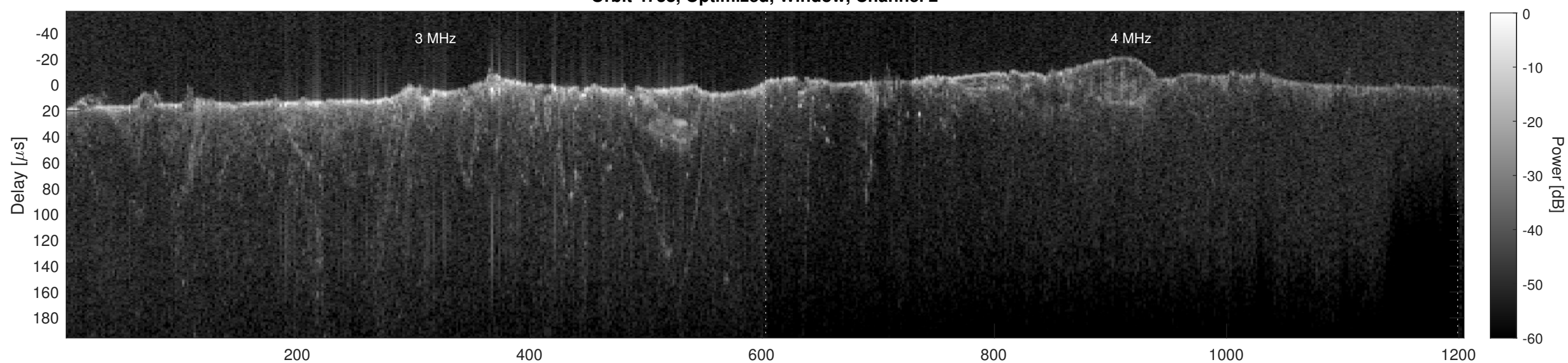
Orbit 4738, Cluttergram
