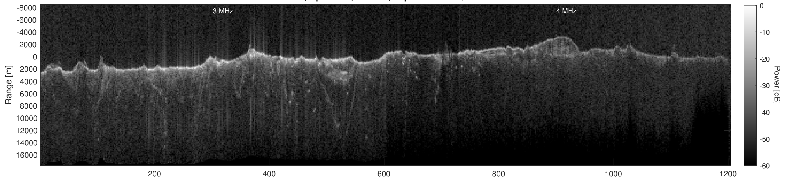
Orbit 4738, Depth-Corrected Cluttergram
