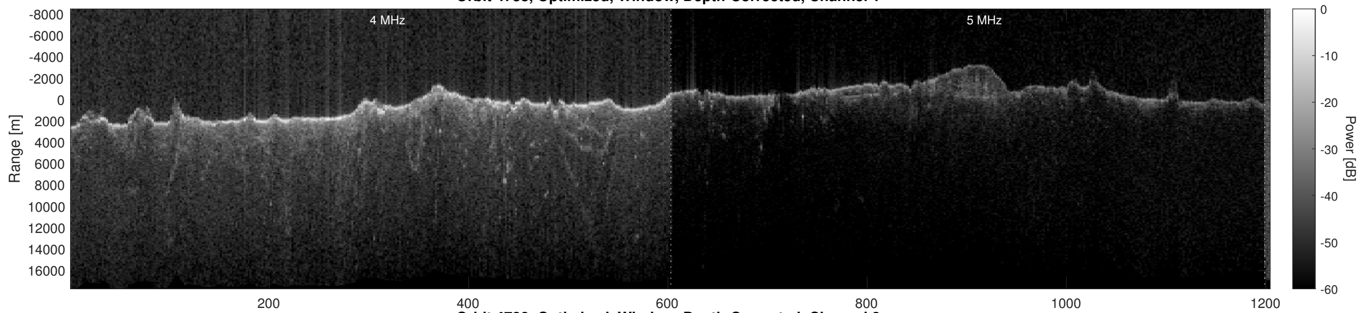
Orbit 4738, Optimized, Window, Depth-Corrected, Channel 2
