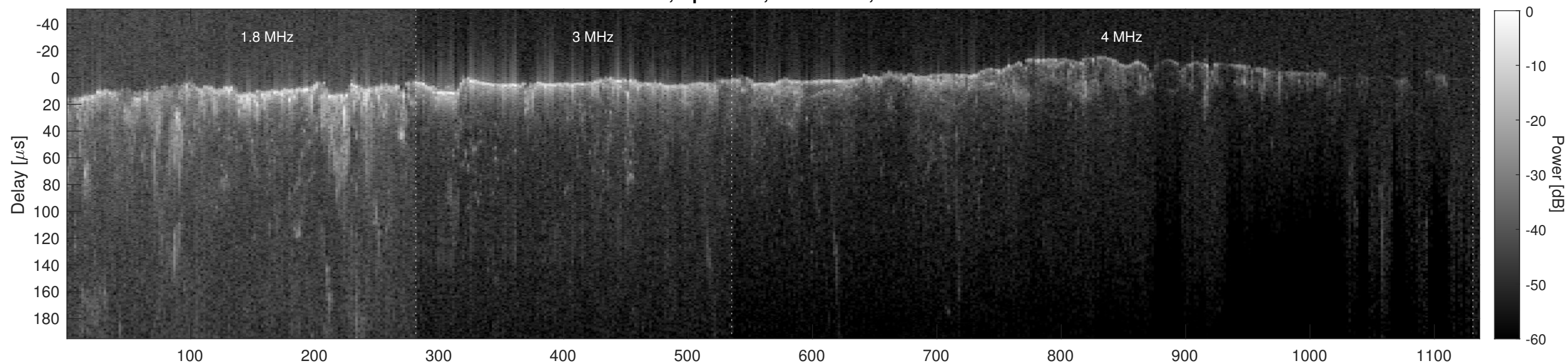
Orbit 4740, Cluttergram
