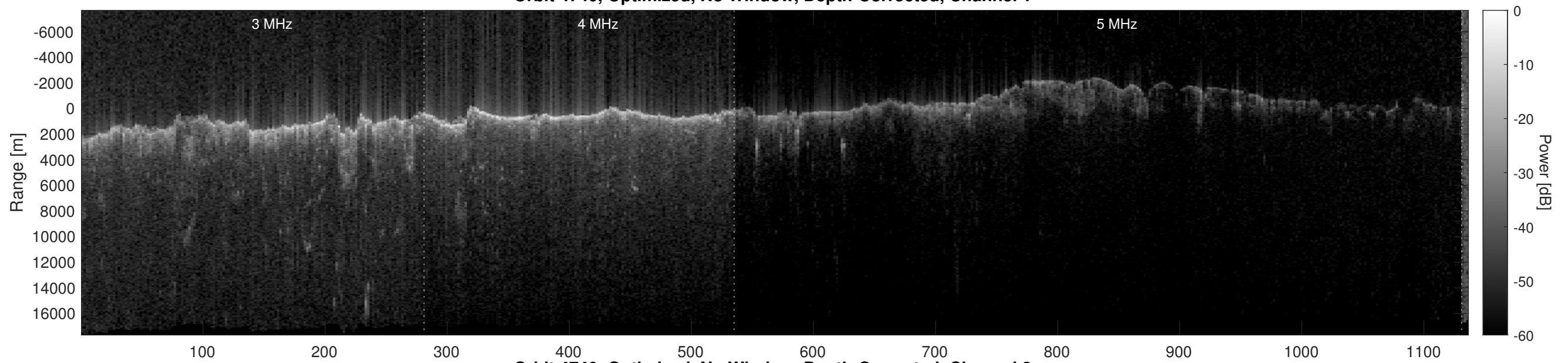
Orbit 4740, Optimized, No Window, Depth-Corrected, Channel 2
