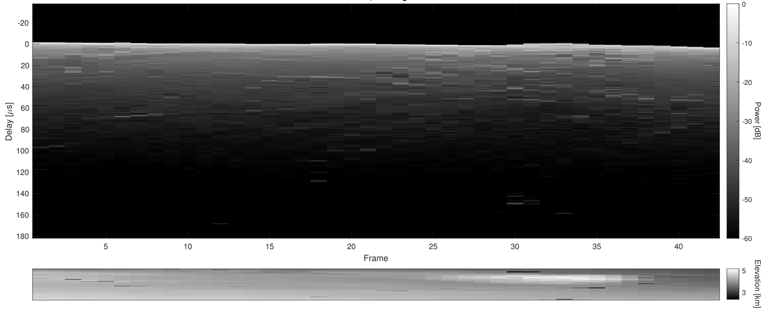
Orbit 4741, Cluttergram
