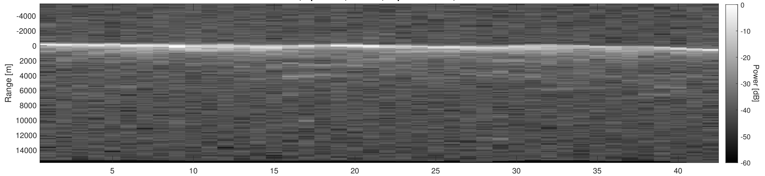
Orbit 4741, Depth-Corrected Cluttergram
