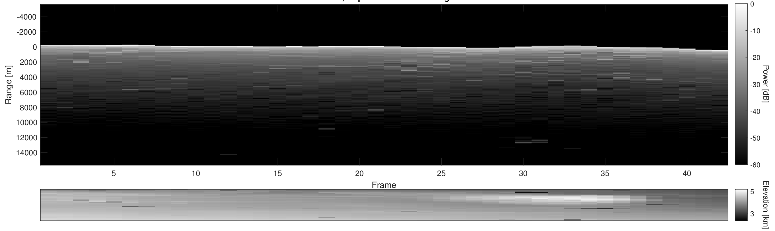
Orbit 4741, Depth-Corrected Cluttergram
