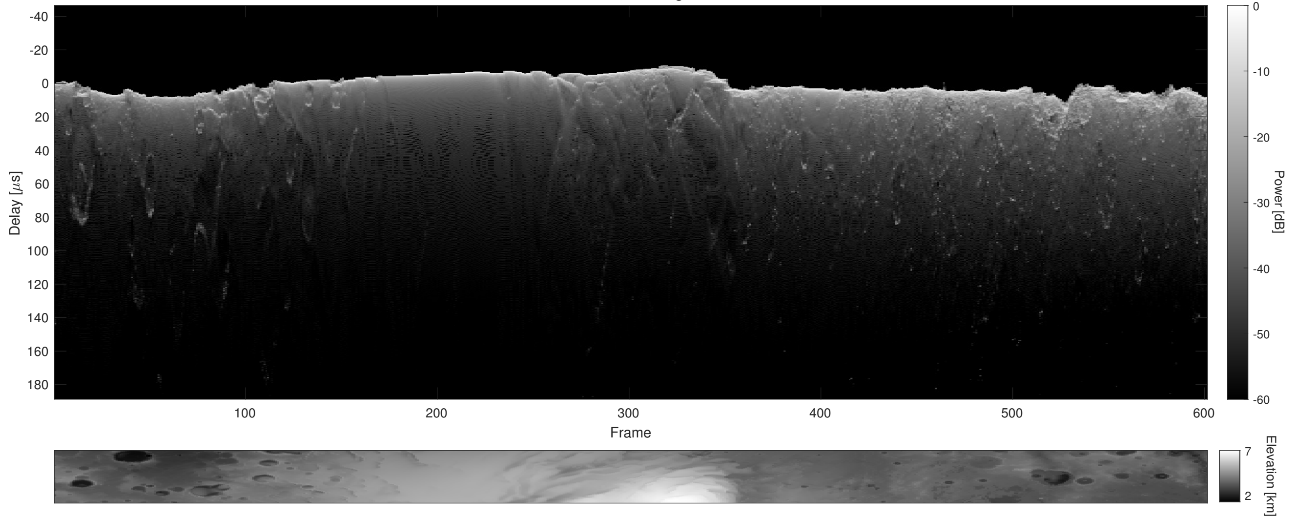
Orbit 4742, Cluttergram
