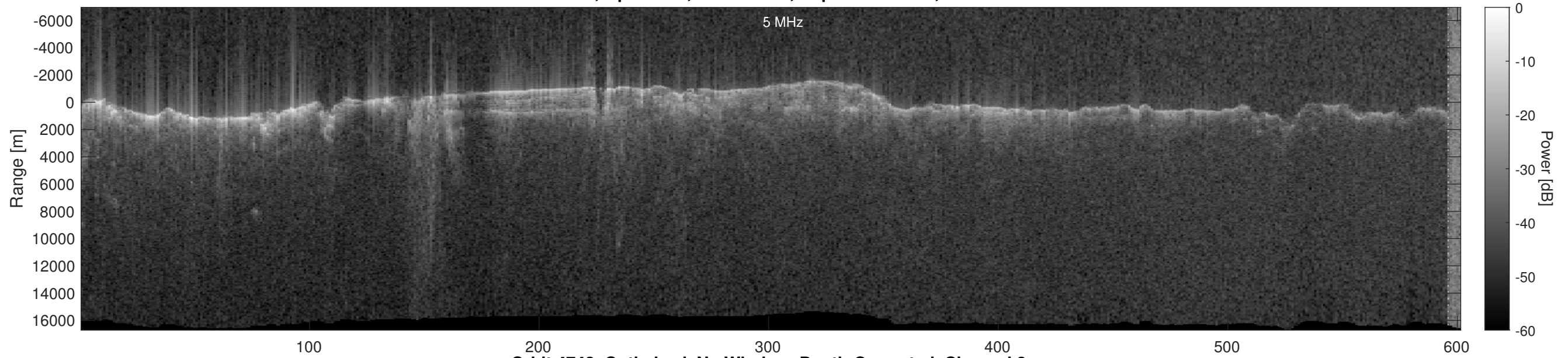
Orbit 4742, Optimized, No Window, Depth-Corrected, Channel 2
