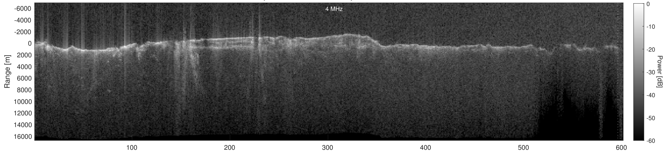
Orbit 4742, Depth-Corrected Cluttergram
