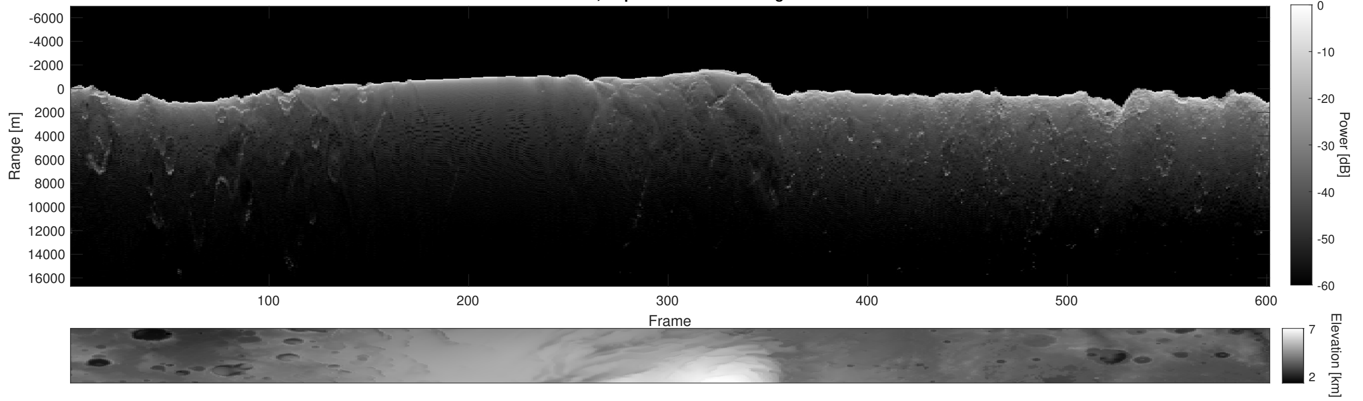
Orbit 4742, Depth-Corrected Cluttergram
