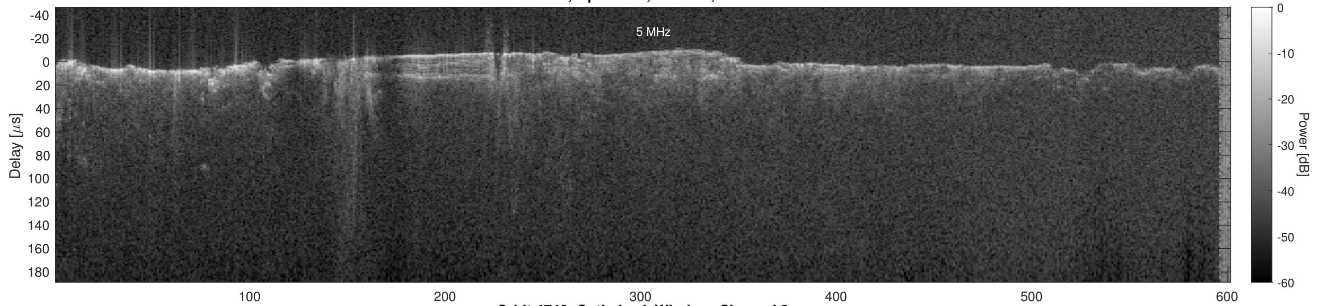
Orbit 4742, Optimized, Window, Channel 2
