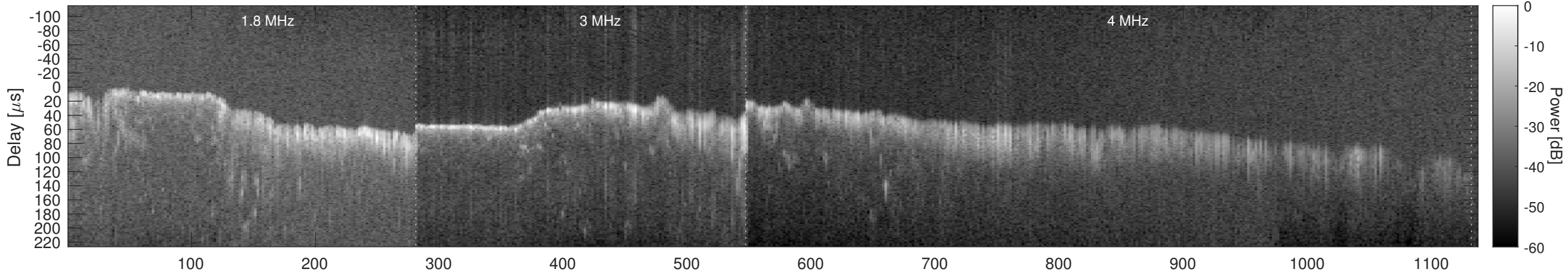
Orbit 4743, Window, Channel 2, Chapman
