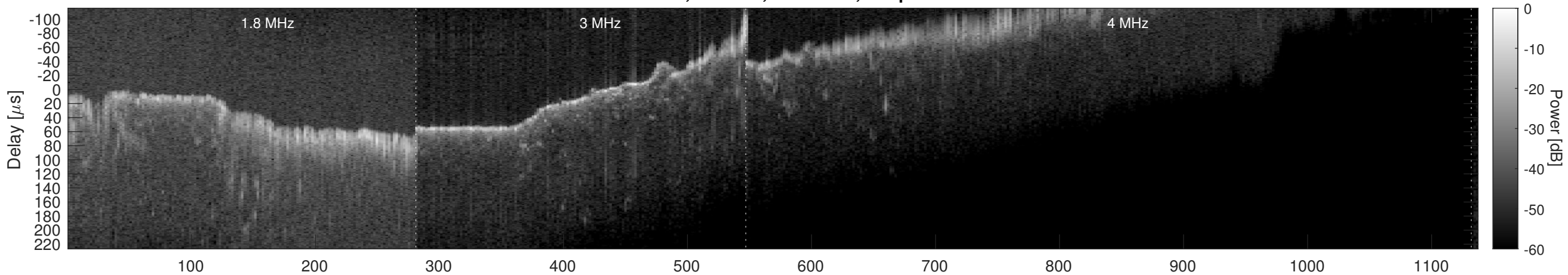
Orbit 4743, Window, Channel 2, Optimized
