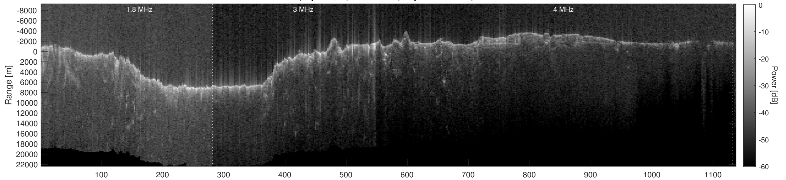
Orbit 4743, Depth-Corrected Cluttergram
