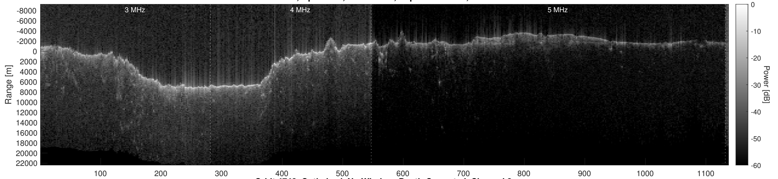
Orbit 4743, Optimized, No Window, Depth-Corrected, Channel 2
