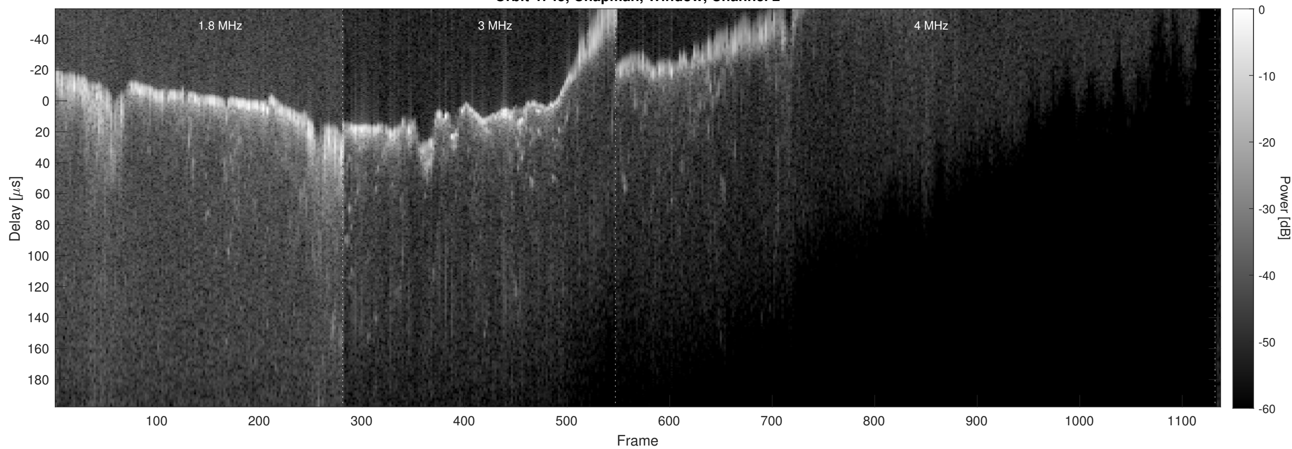
Orbit 4745, Chapman, Window, Channel 2
