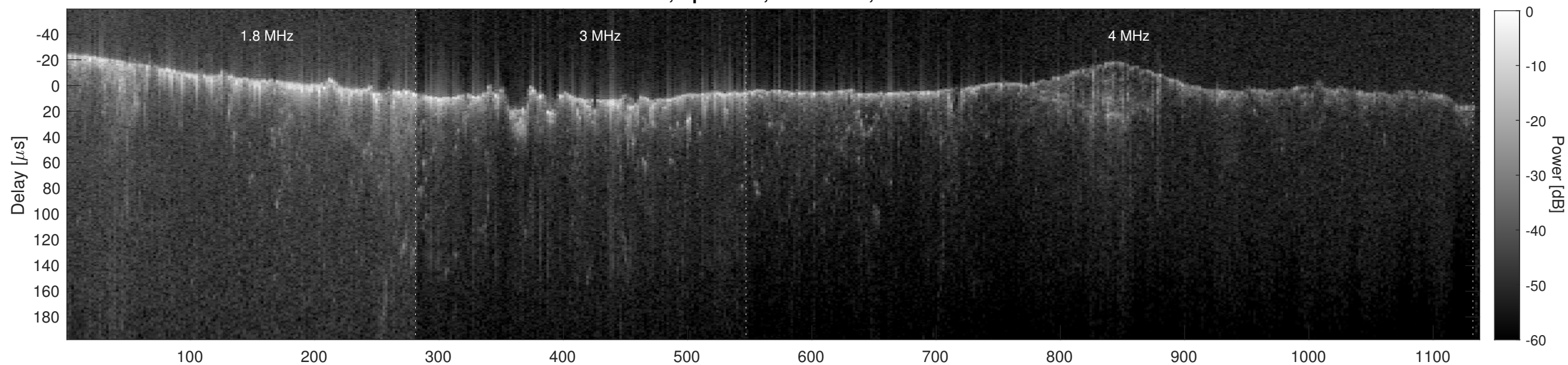
Orbit 4745, Cluttergram
