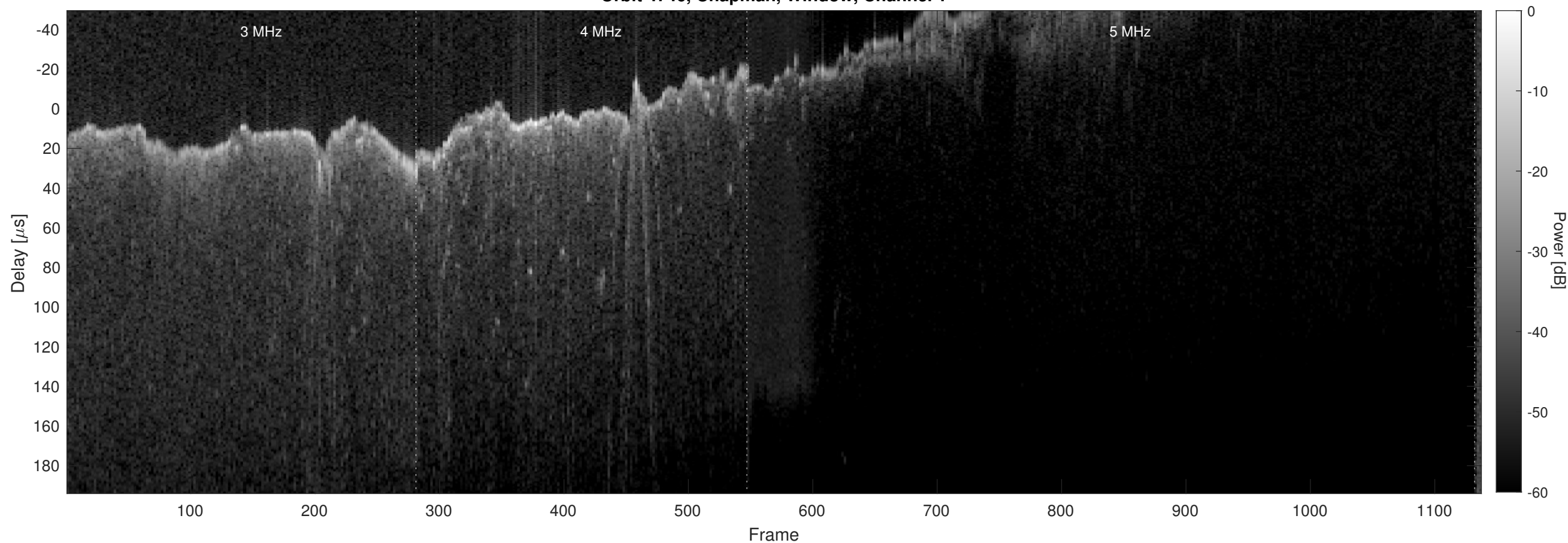
Orbit 4746, Chapman, Window, Channel 2
