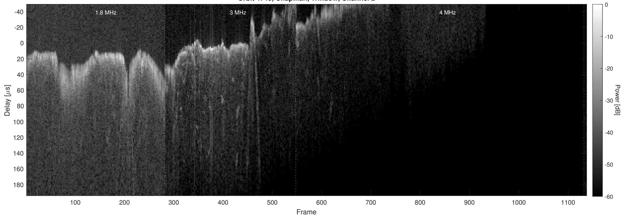
Orbit 4746, Chapman, Window, Channel 2
