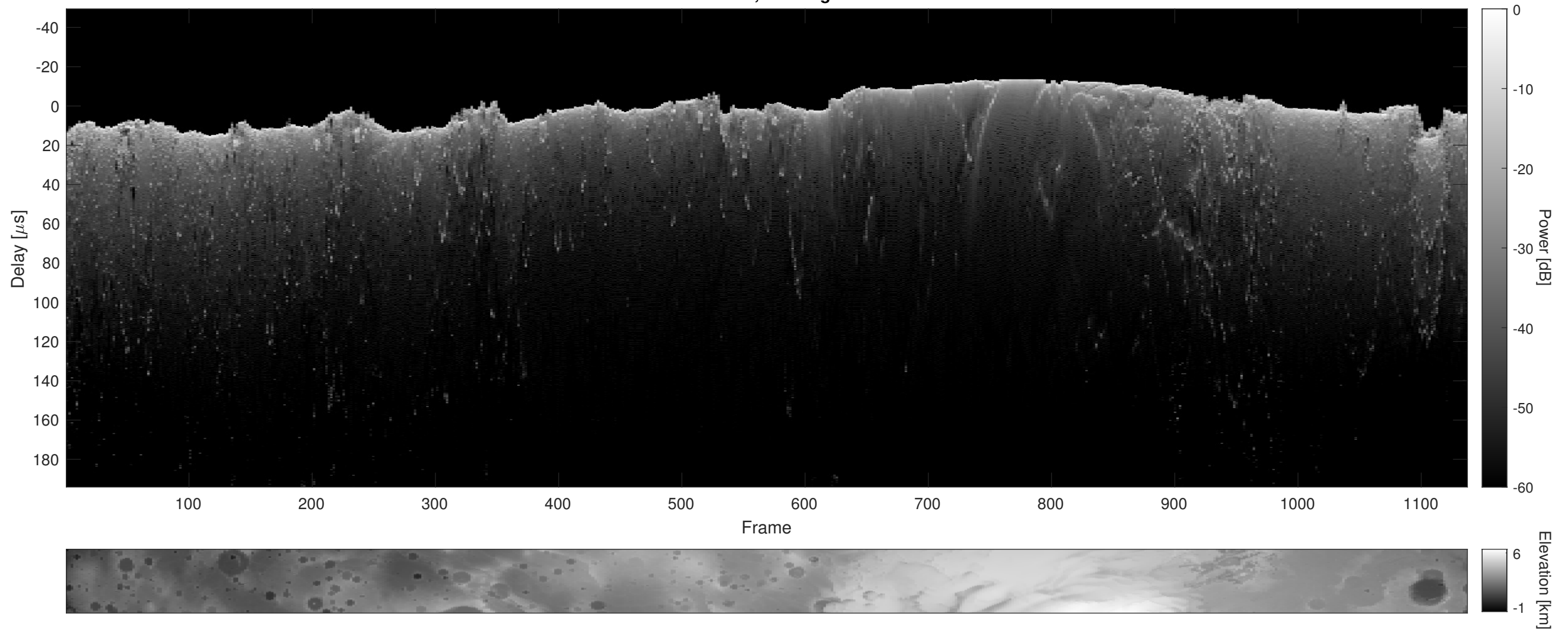
Orbit 4746, Cluttergram
